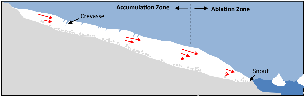
Cross Section of a Valley Glacier
